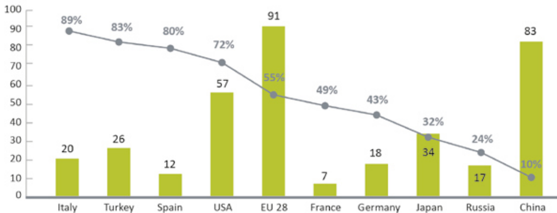
Steel scrap volume – absolute and as a percentage per tonne of crude steel produced
