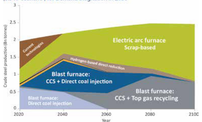
Technology competition in the binding climate target scenario (3.5 RF scenario) for Demand Stagnation in 2050
